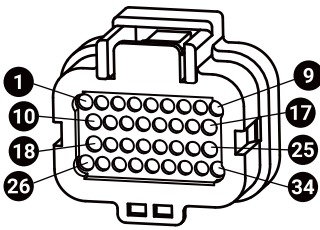
SUPERSEAL 1.0 4-1437290-1 34 POS
