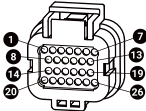
SUPERSEAL 1.0 1473416-1 26 POS
